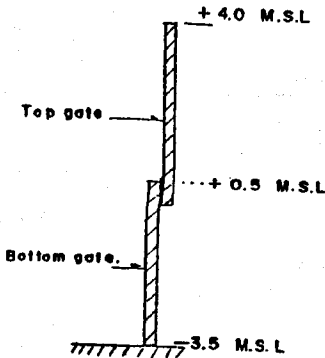
18 No/20 ft. Span gates Clear length = 360 ft
