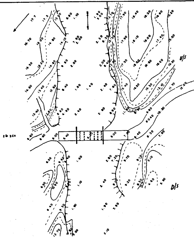
SITE SURVEY OF CAUSEWAY AT 2 M 3.0 CH
