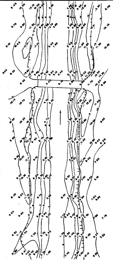
SITE SURVEY OF REGULATOR CUM CAUSEWAY AT OM. 27.0 CHS SCALE : 40 FT TO AN INCH
