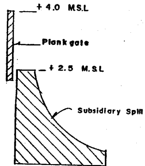
16 No/10 ft Span gates Clear Spill length = 160 ft.
