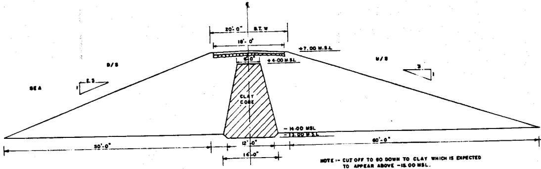
SECTION C-C SCALE 1" = 10 FT TO AN INCH
